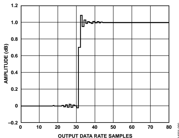
Figure 90. Wideband Filter Step Response
