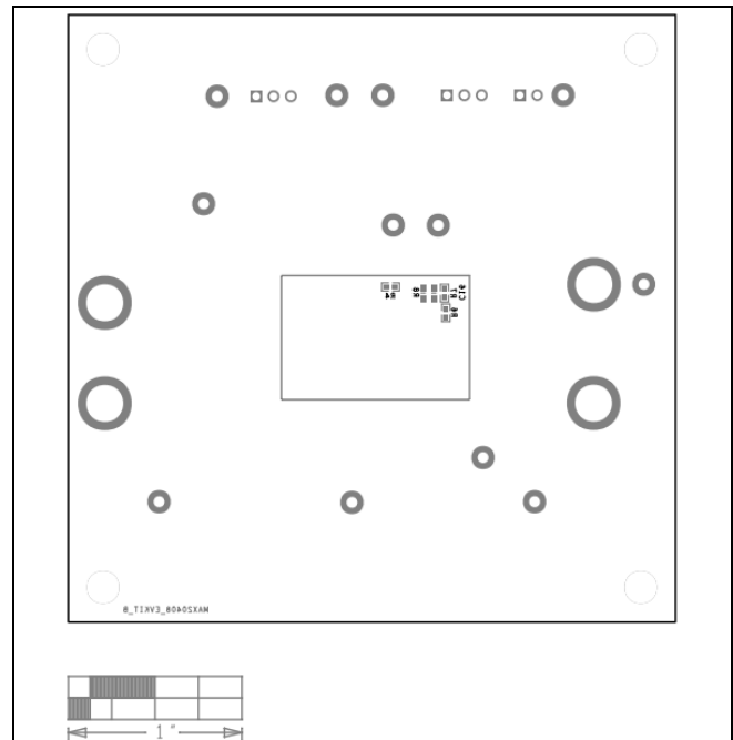
MAX42410 EV Kit Component Placement Guide—Bottom Silkscreen
